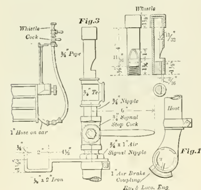
"BACK-UP" HOSE AND CONNECTIONS USED ON THE CHICAGO & NORTH-WESTERN R.R.
